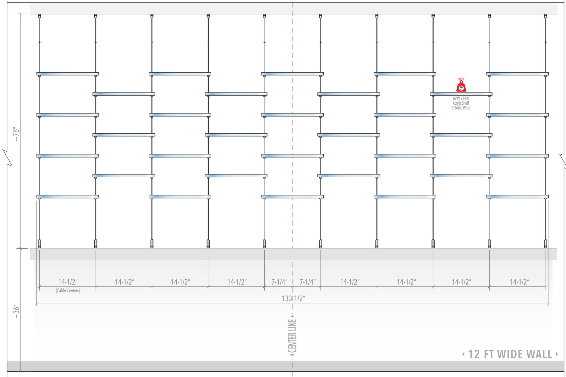
Front View
