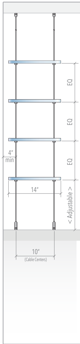
Side View
